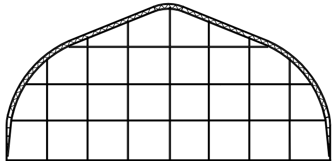
Plain End
